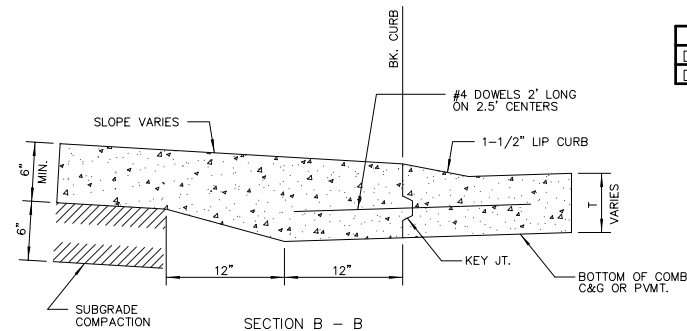
FULL RAMP DRIVE (P = 4.0' TO 6.5')
