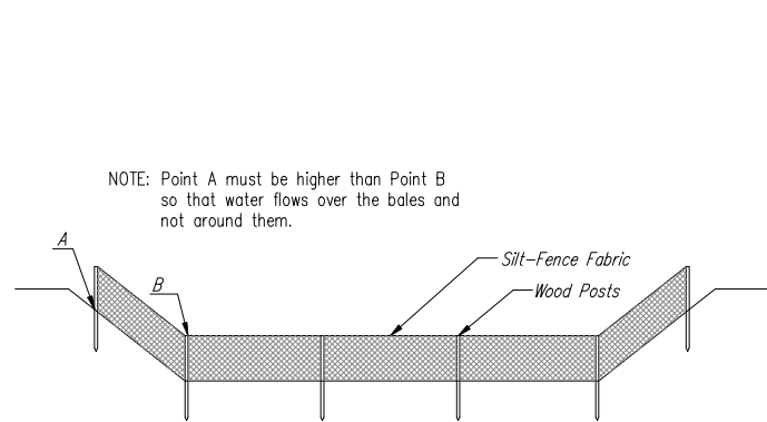
SILT FENCE DITCH CHECKS (STREAM PROTECTION)
