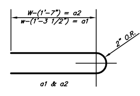
BENDING DIAGRAM
