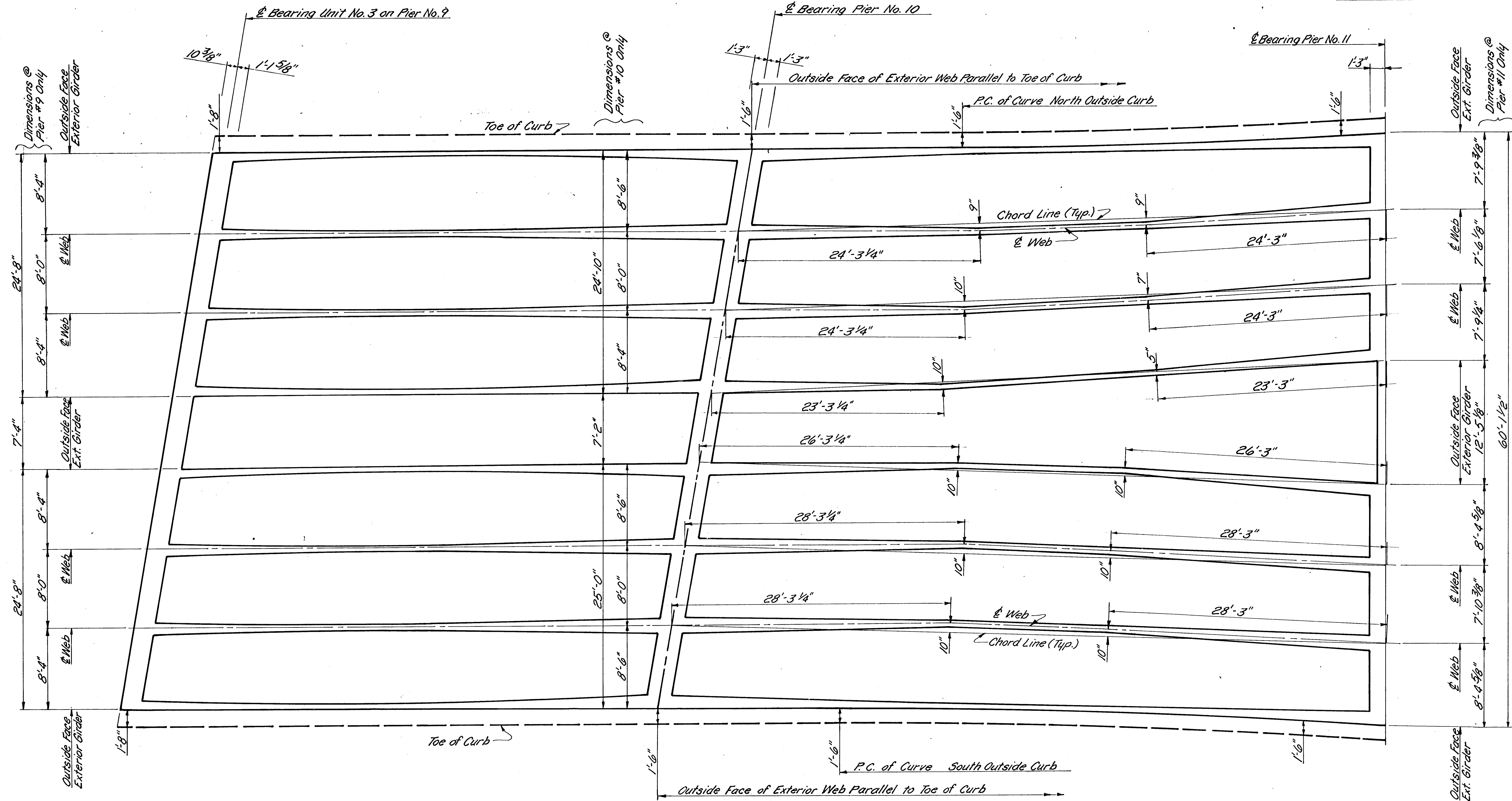
UNIT NO. 3 - SPANS 1 & 2 (Showing Web Location)
