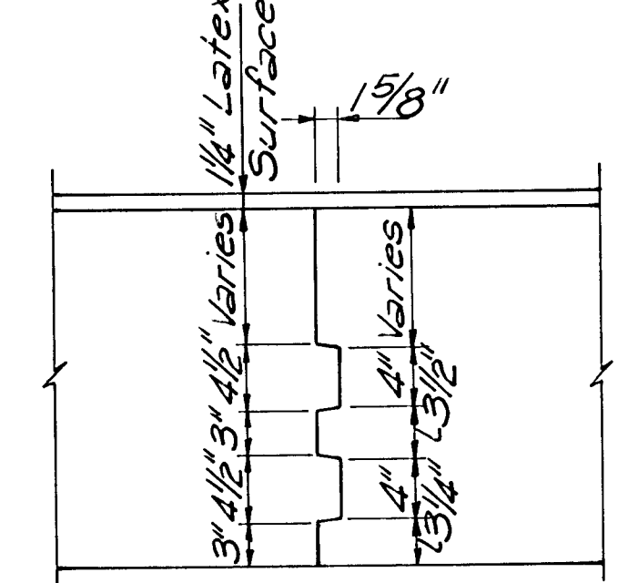
TRANSVERSE SLAB CONSTRUCTION JOINT
