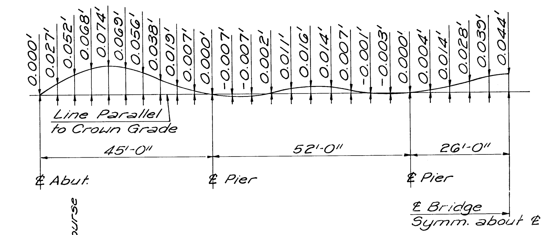
DEAD LOAD CAMBER AT TENTH POINTS
