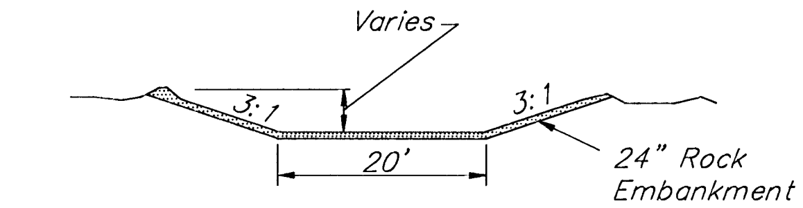
Diagram of a trapezoidal channel cross-section. The bottom width is 20'. The side slopes are 3:1. The water depth is labeled "Varies".
