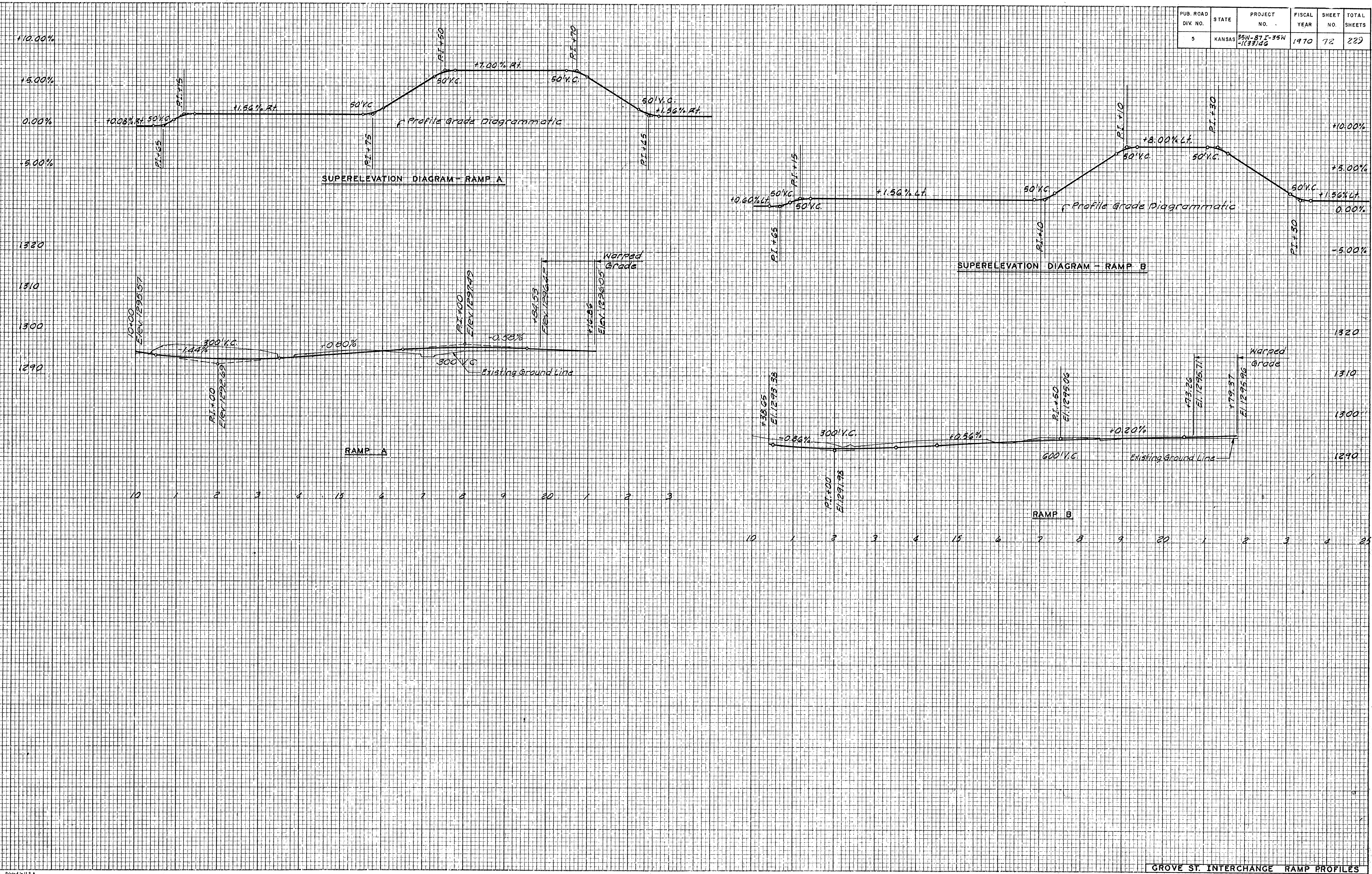
GROVE ST. INTERCHANGE RAMP PROFILES
