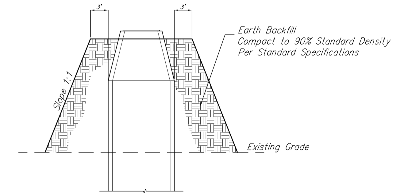
FILL PLACEMENT DETAIL (To be paid for as "Easement Grading - L.S.")
