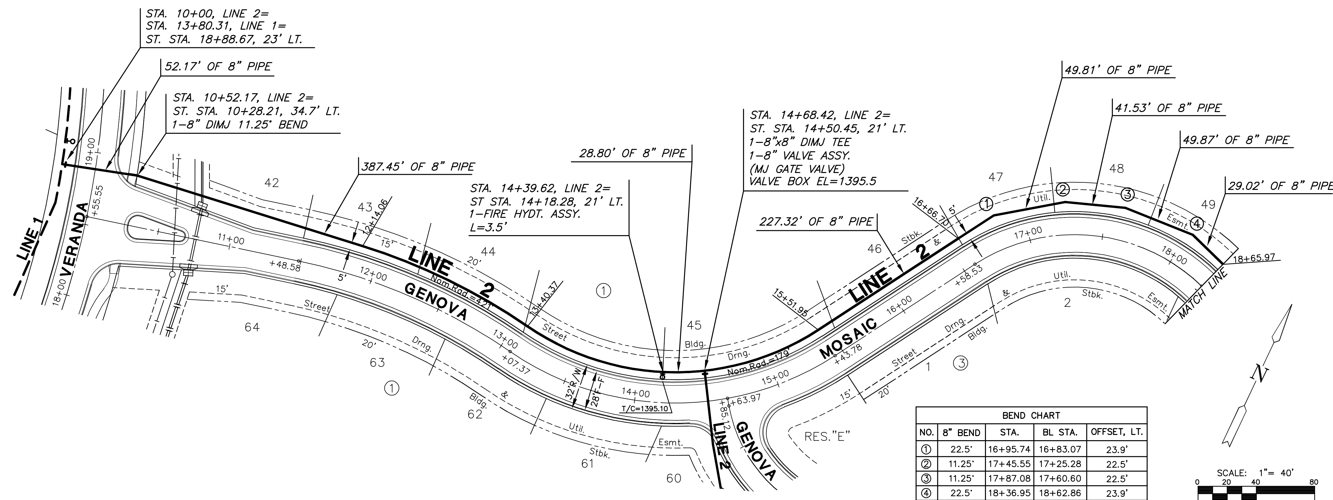
PLAN LINE 2 PROFILE LINE 2
