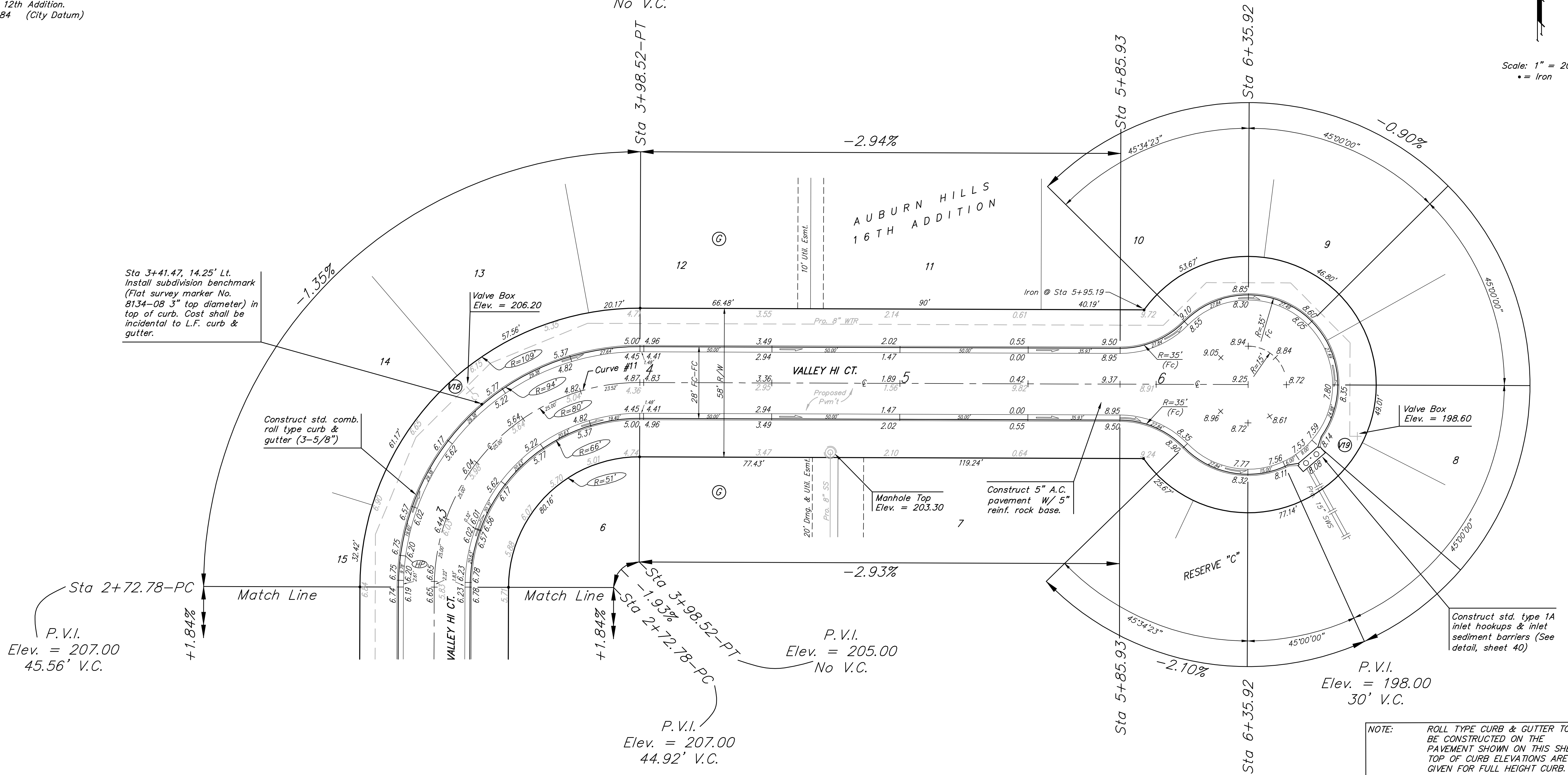
Curve #11 Curve Data Based on Centerline Rad. = 80' Delta = 90°03'26" Tangent = 80.08' Arc = 125.74' L.C. = 113.19' Def./Fl. = 21.48653 Min.
