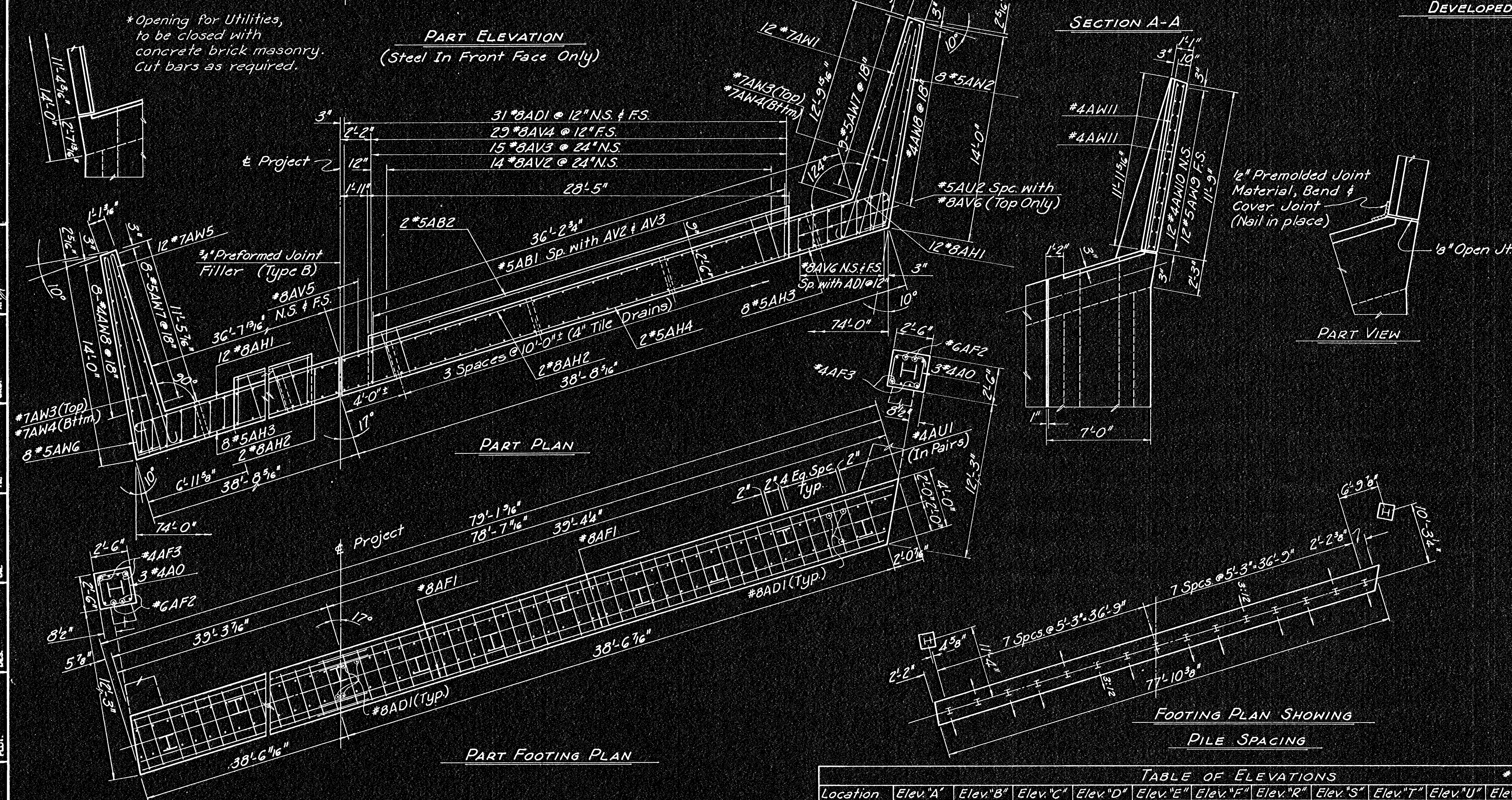
DEVELOPED VIEW WING WALL
