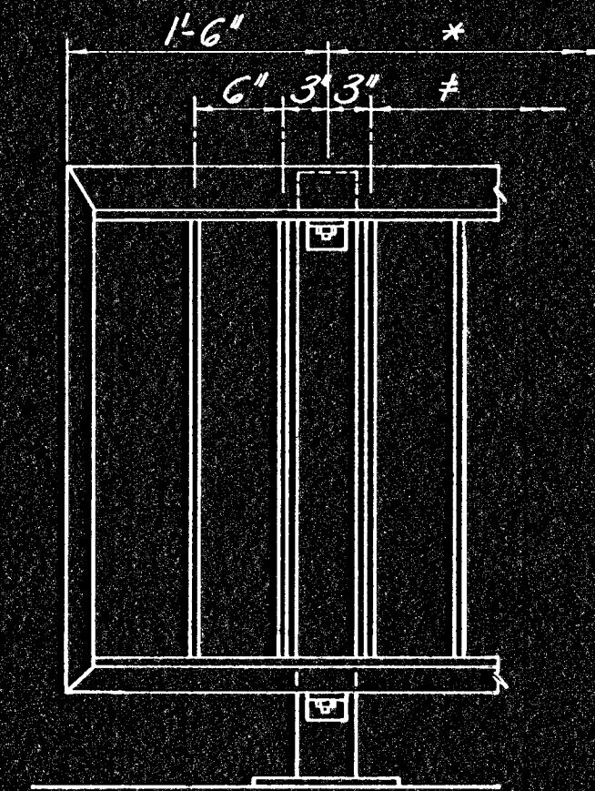
Note: All parts of Metal Handrail, posts, base plates and rail, shall be fabricated from A-36 steel. Painting: Shop and field coats shall conform to the basic lead silico cromate system.
