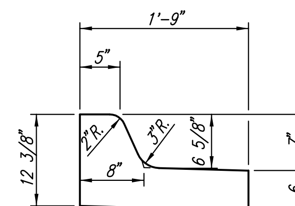
MEDIAN COMBINED CURB & GUTTER (6 5/8")
