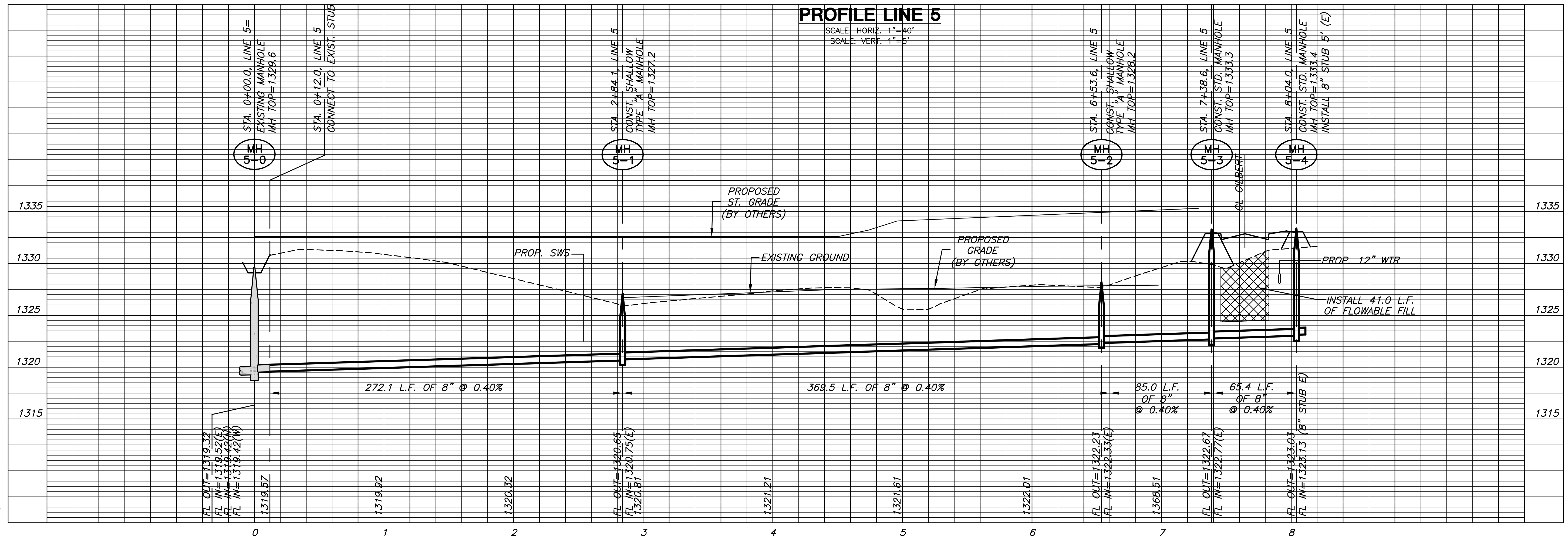
PLAN LINE 5 SCALE: 1"=40'
