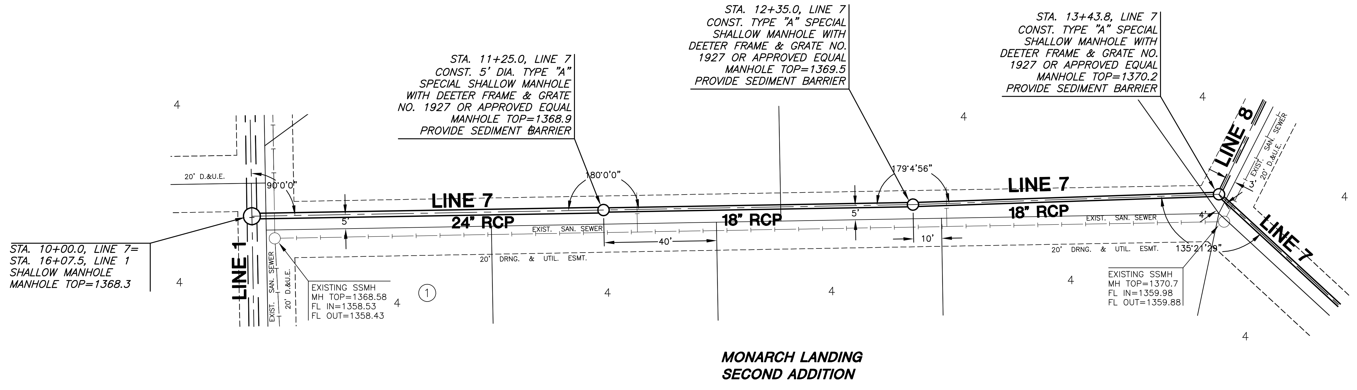
PLAN LINE 7
