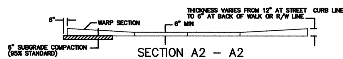
FULL RAMP DRIVES (P = 4.0' & 6.5')
