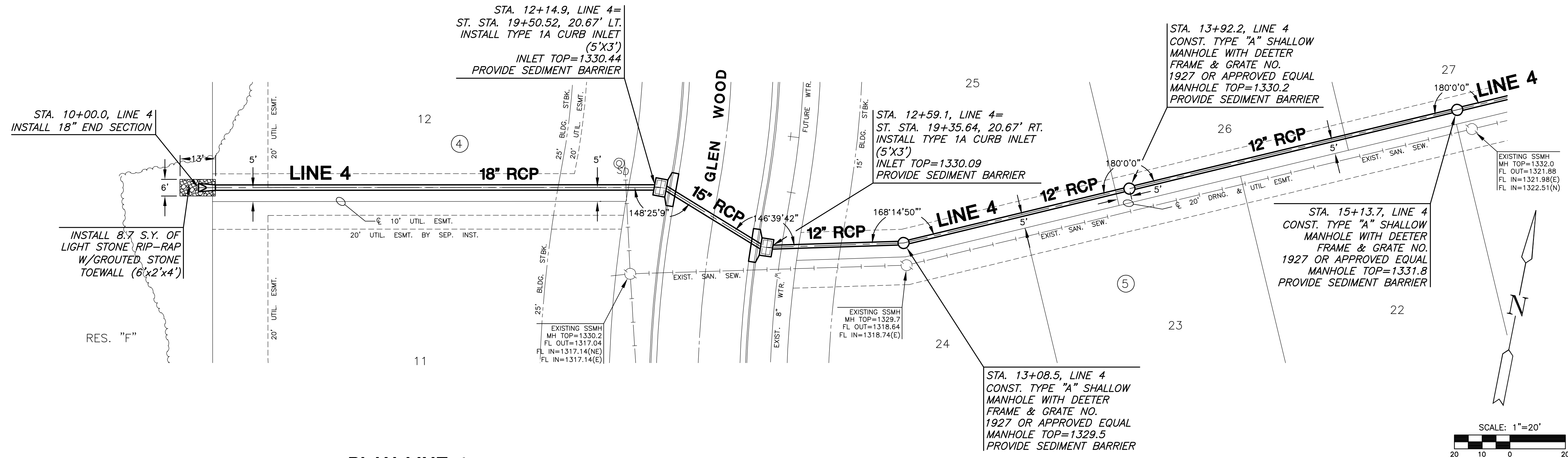
PLAN LINE 4
