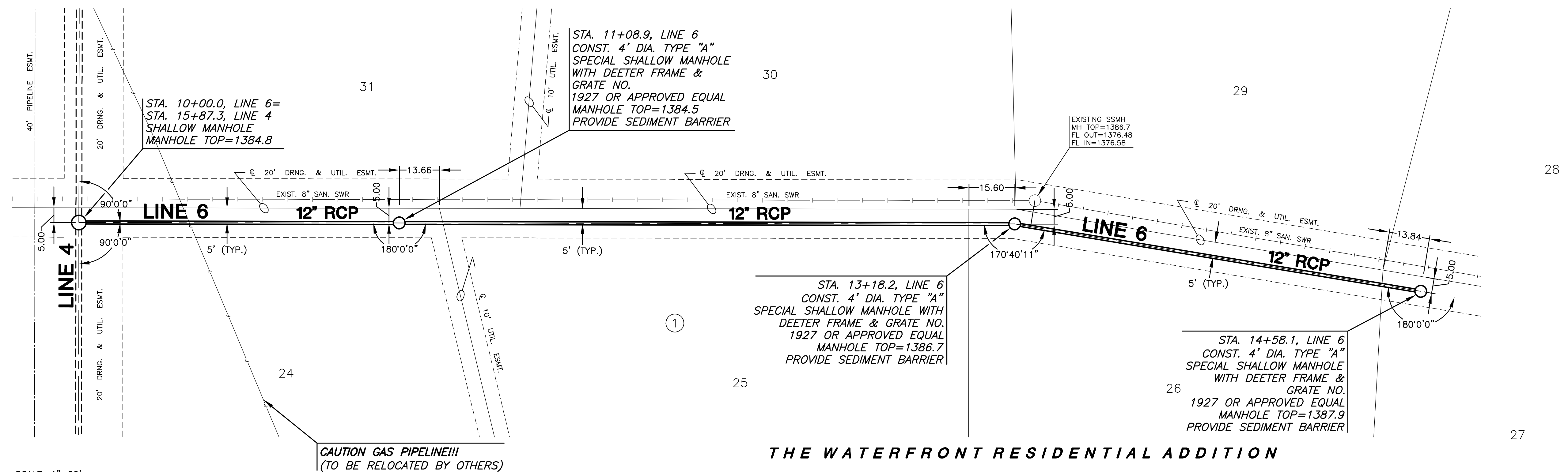
PLAN LINE 6
