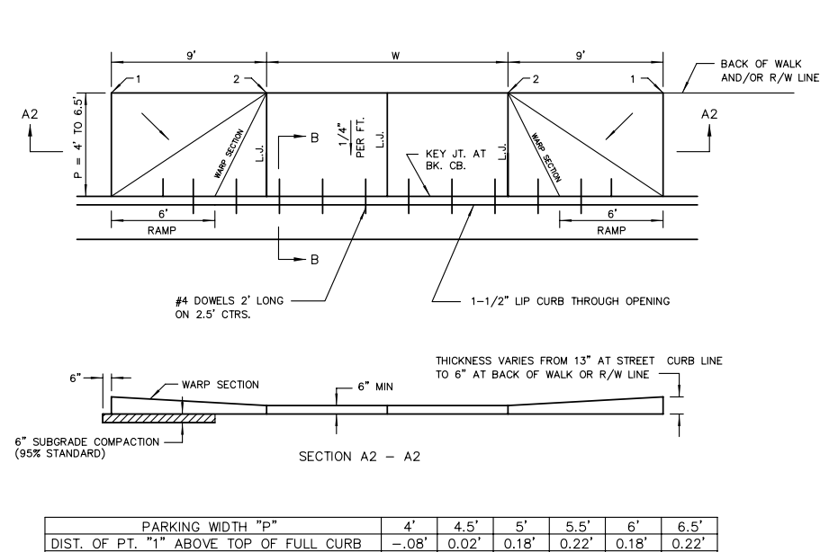
FULL RAMP DRIVE (P = 4.0' TO 6.5')
