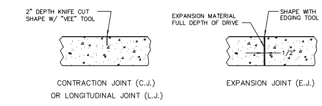
CONTRACTION JOINT (C.J.) OR LONGITUDINAL JOINT (L.J.)
