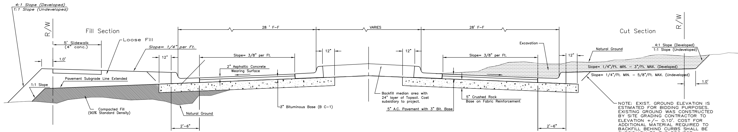
TYPICAL MEDIAN SECTION
