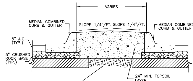
MEDIAN DETAIL SCALE: NONE
