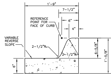
MEDIAN COMBINED CURB & GUTTER (6-5/8") SCALE: NONE
