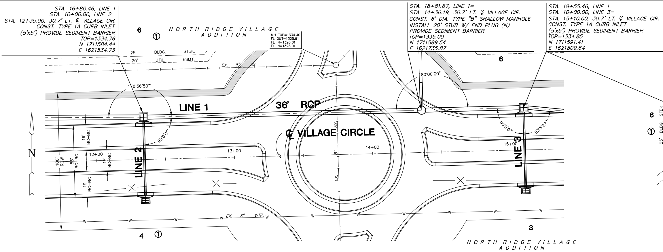
CONT. PLAN LINE 1 SCALE: 1"=20'
