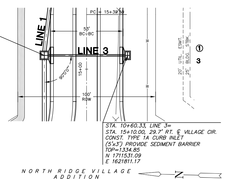
PLAN LINE 3 SCALE: 1"=20'
