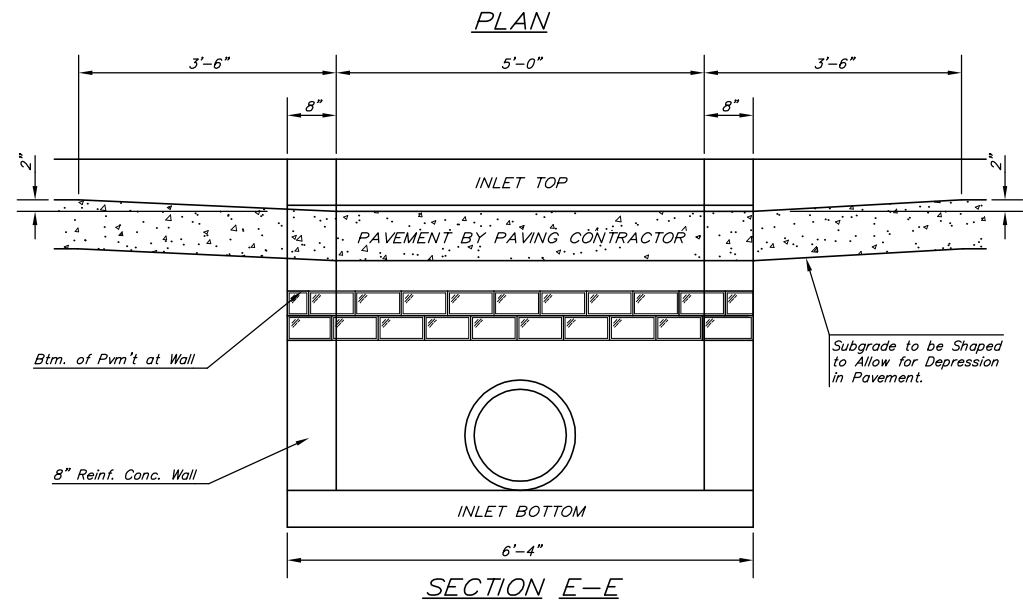
SECTION E-E
