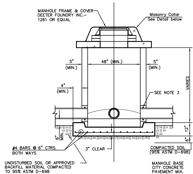
SHALLOW TYPE "P" MANHOLE
