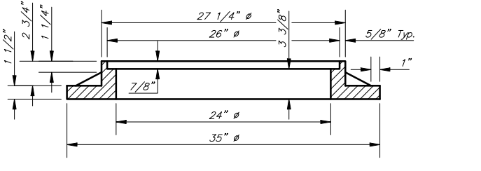
MANHOLE RING AND COVER
