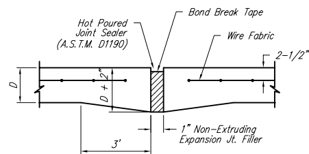
EXPANSION JOINT
