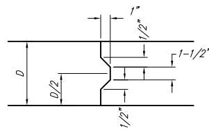
KEYWAY DETAIL
