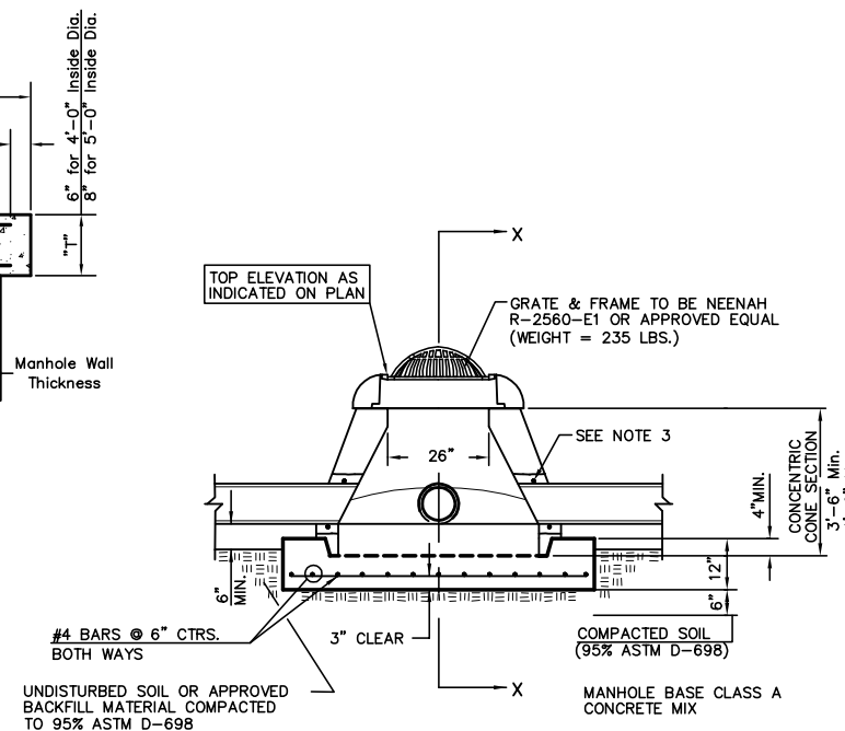
SPECIAL SHALLOW TYPE "P" MANHOLE WITH BEEHIVE FRAME & GRATE
