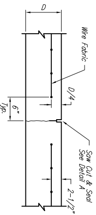
CONTRACTION JOINT DETAIL (C.J.)
