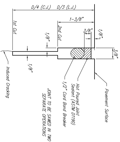
SAW JOINT DETAIL
