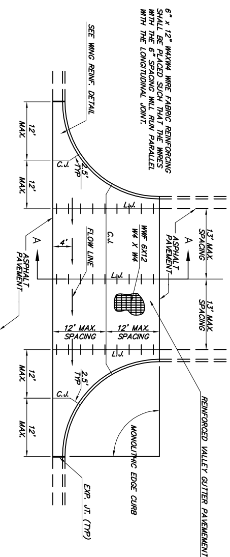
PLAN
