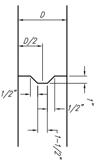
KEYWAY DETAIL
