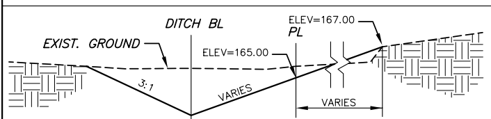
TYPICAL DITCH SECTION
