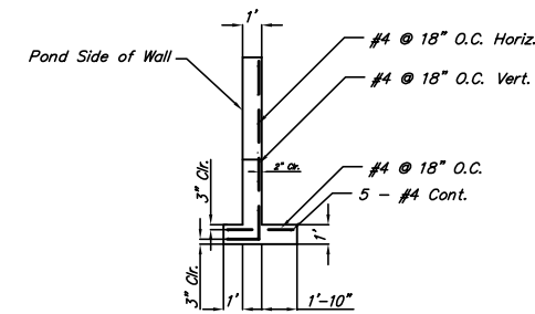
SECTION VIEW
