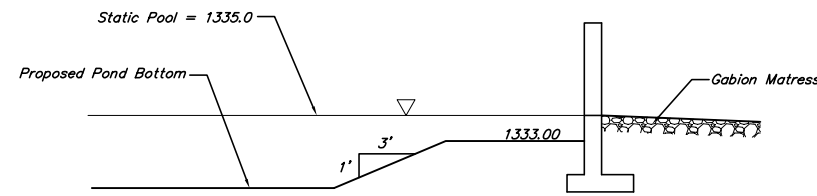
SECTION GRADING DETAIL
