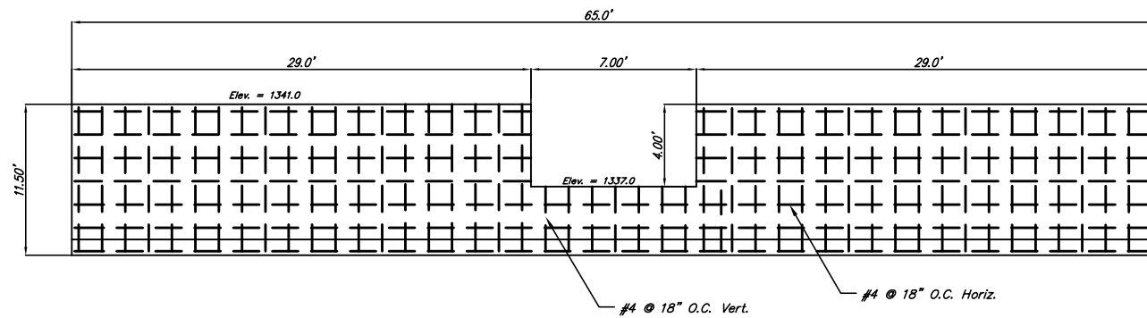
POND #1 WEIR WALL DETAIL
