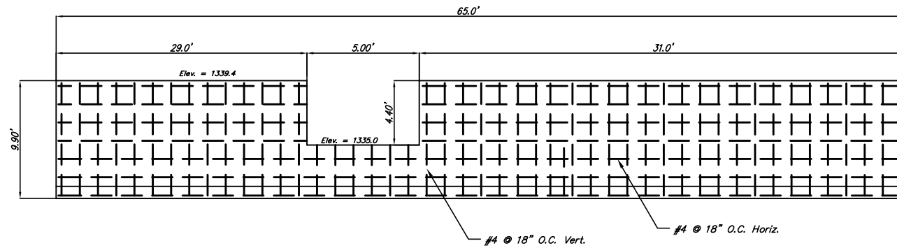
POND #2 WEIR WALL DETAIL
