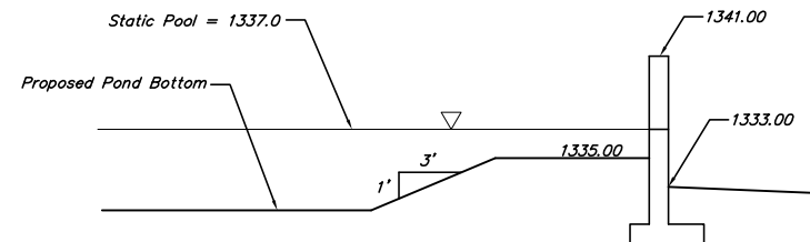
SECTION GRADING DETAIL
