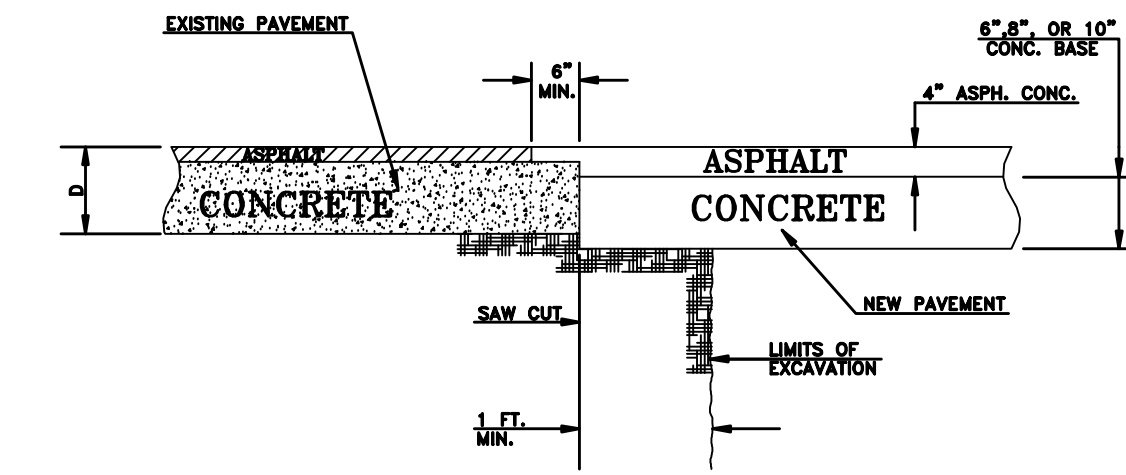
UTILITY CUT REPAIR (ASPHALT CONCRETE PATCH)
