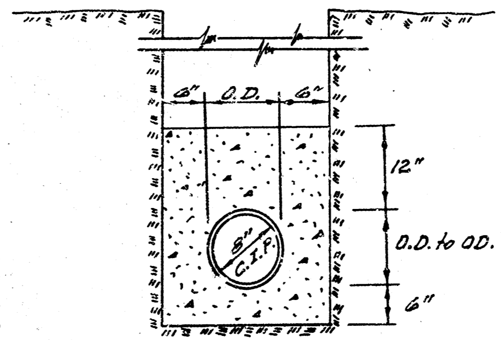
DETAIL OF ENCASEMENT UNDER TRACKS
