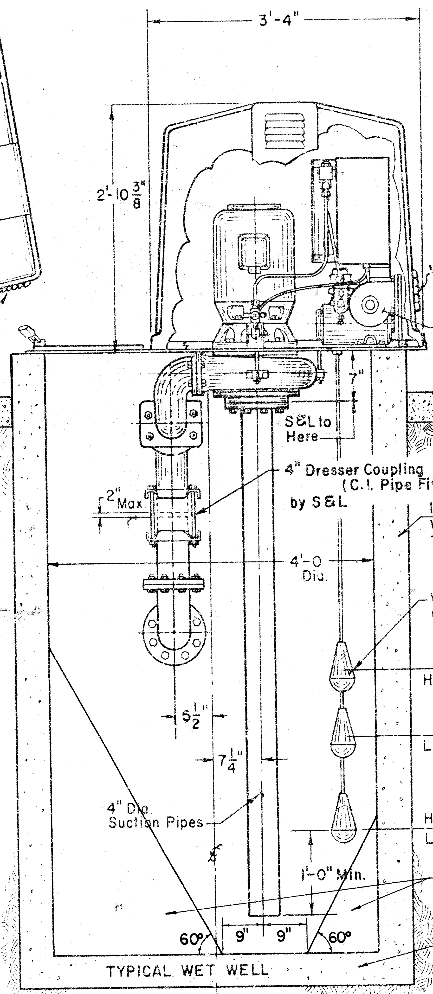
CROSS SECTION
