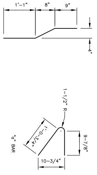
BENDING DIAGRAM
