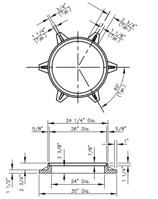
CAST IRON MANHOLE RING
