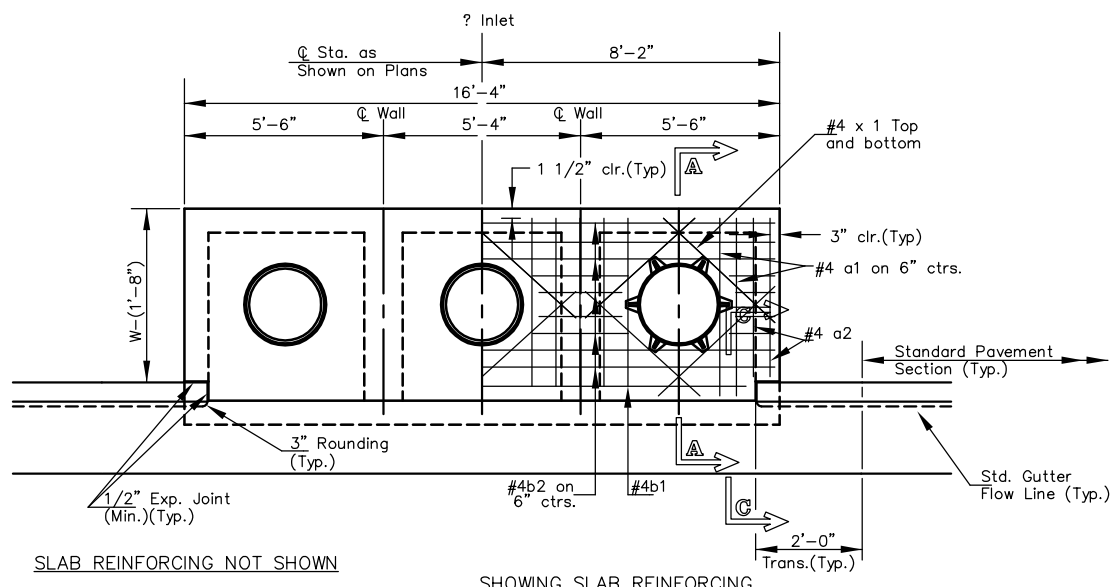
PLAN
