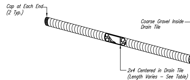
CURB INLET PROTECTION 4" PERFORATED PIPE W/ GRAVEL
