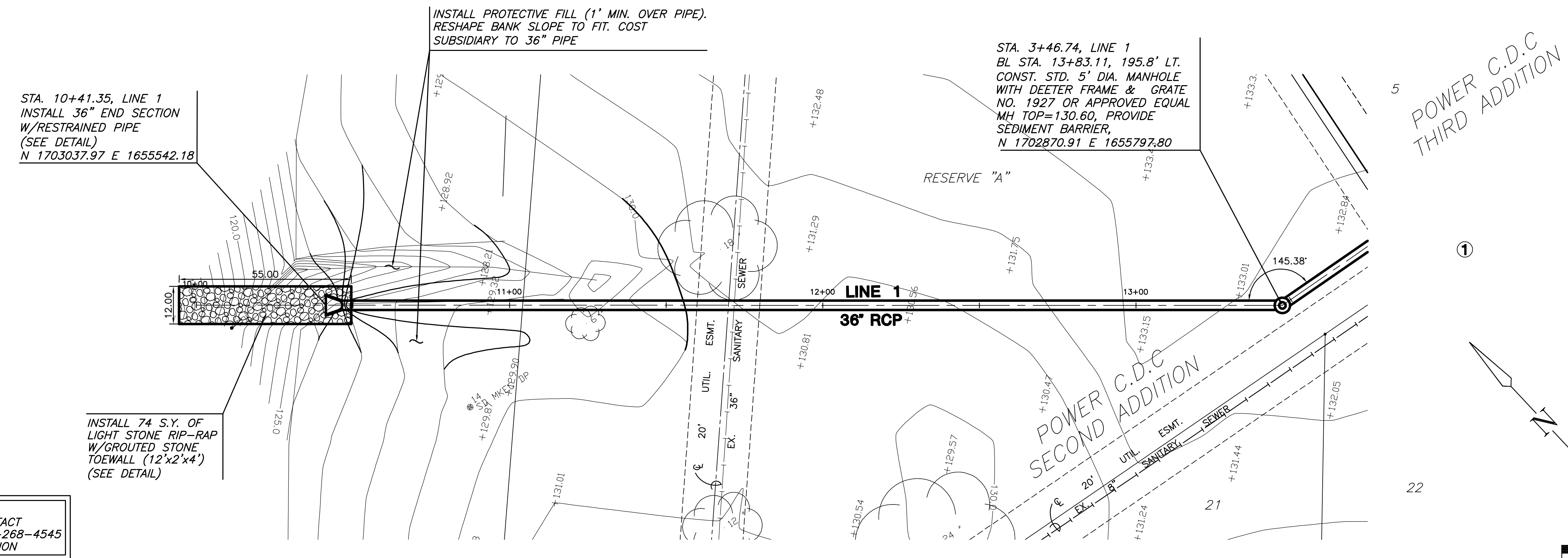
PLAN - LINE 1 SCALE: 1" = 20'
