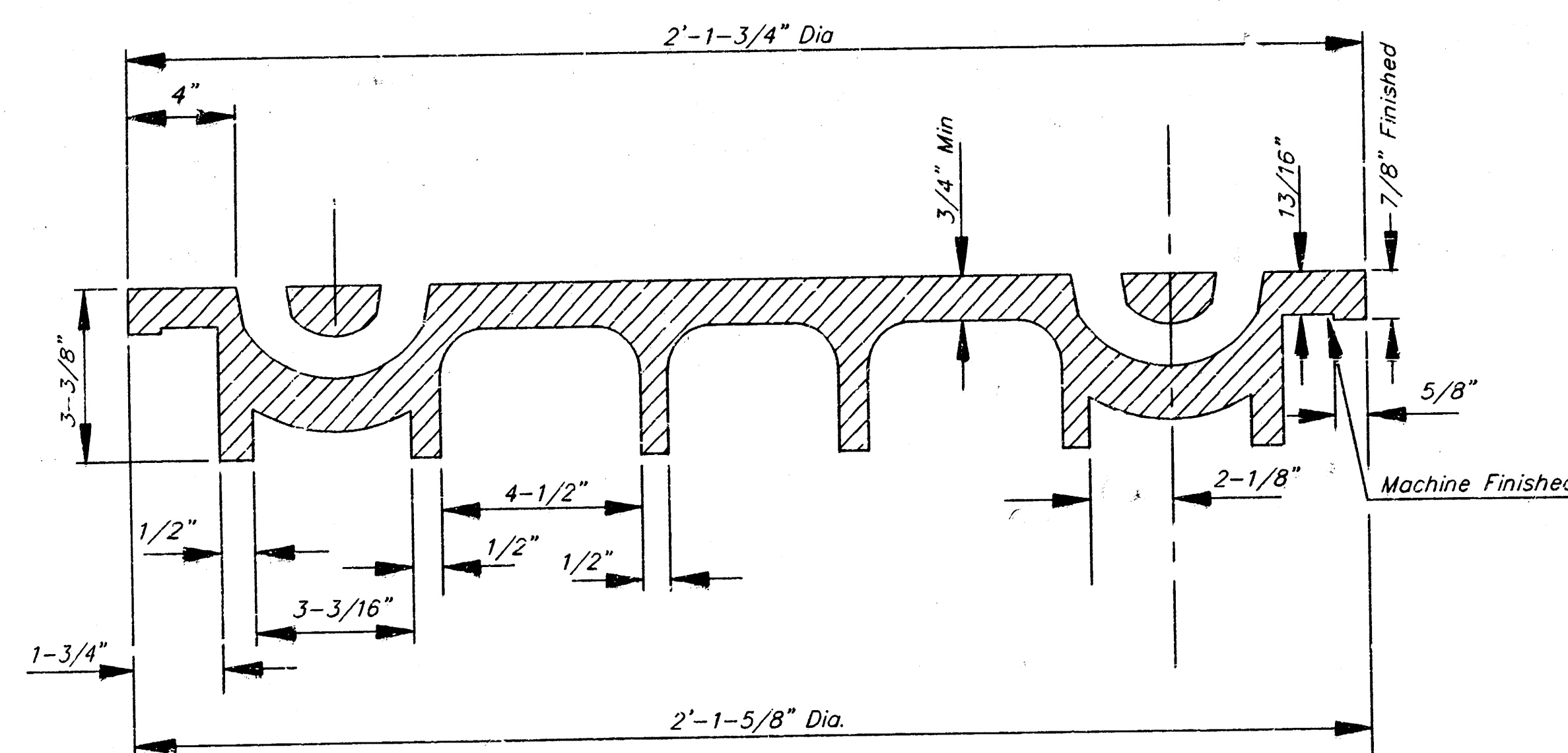
SECTION VIEW
