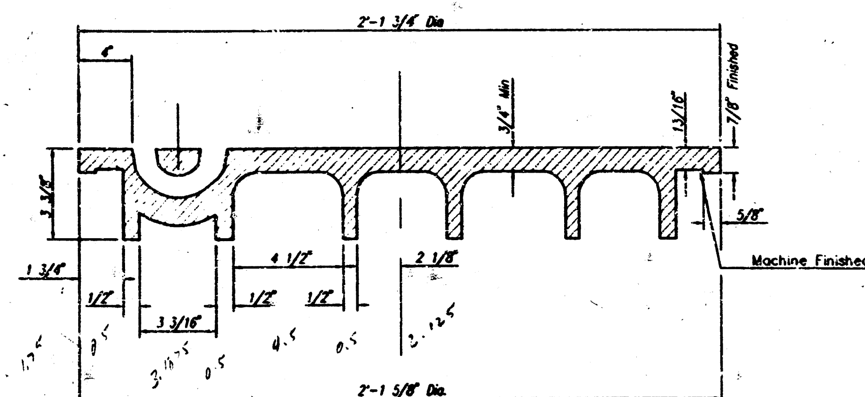
SECTION VIEW
