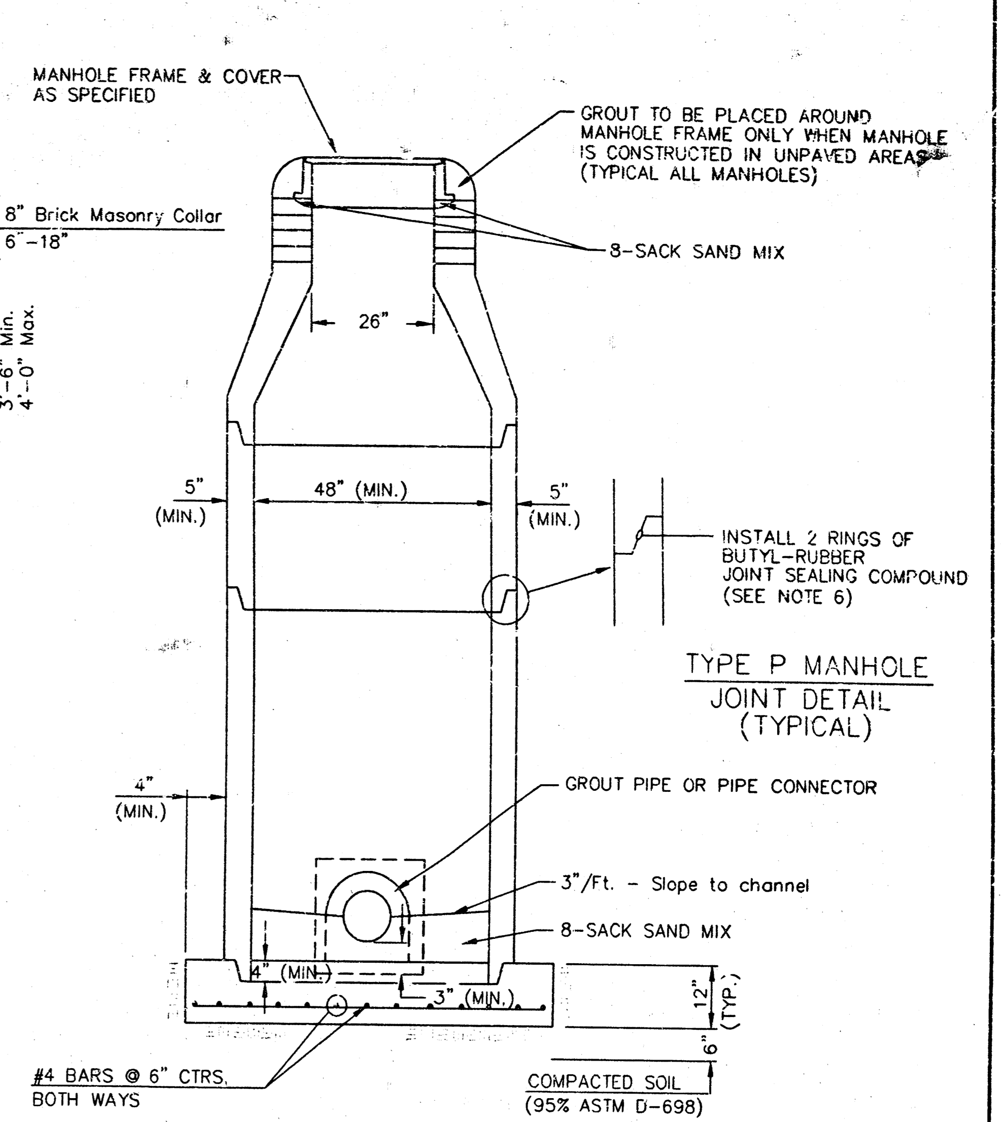
TYPE P MANHOLE JOINT DETAIL (TYPICAL)
