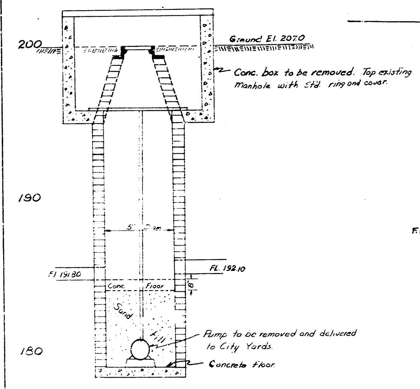
DETAILS FOR REMODELING MANHOLE 30+46
