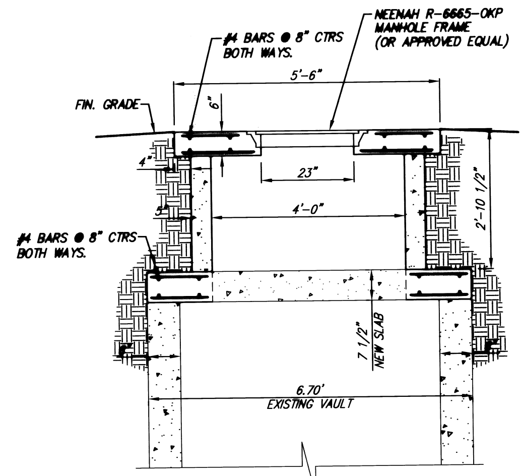
SECTION A-A PRESSURE VAULT DETAIL
