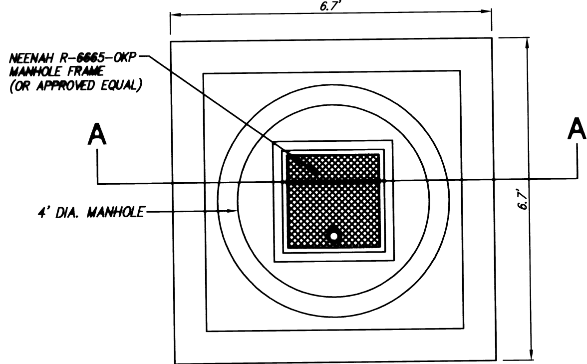
PLAN PRESSURE VAULT DETAIL
