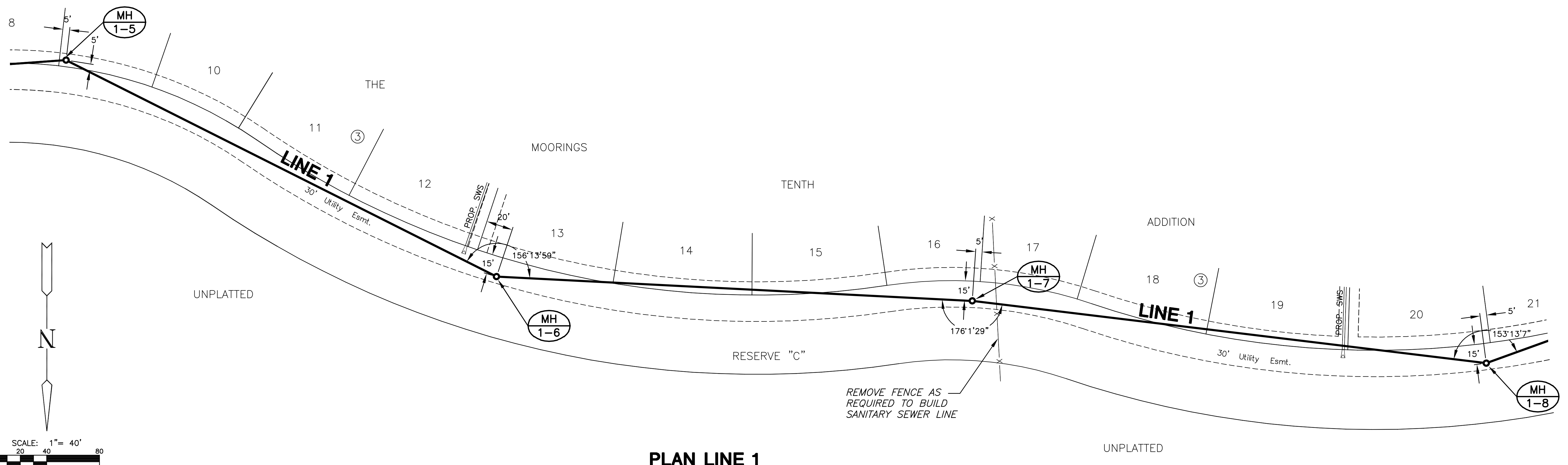
PLAN LINE 1
