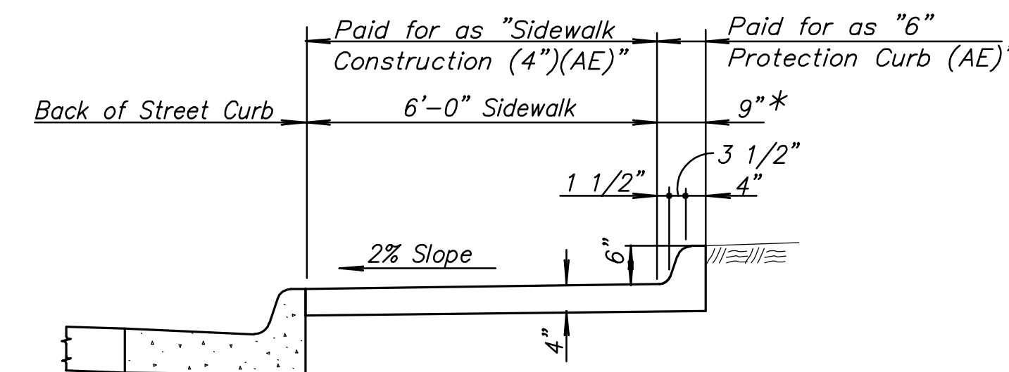
SECTION * Transition as shown at ends
