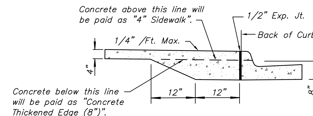
SECTION B1-B1 SIDEWALK SECTION AT BACK-OF-CURB
