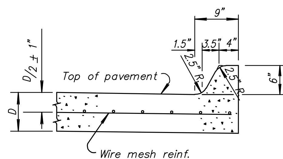
TYPICAL SECTION 6" EDGE CURB (MONOLITHIC)
