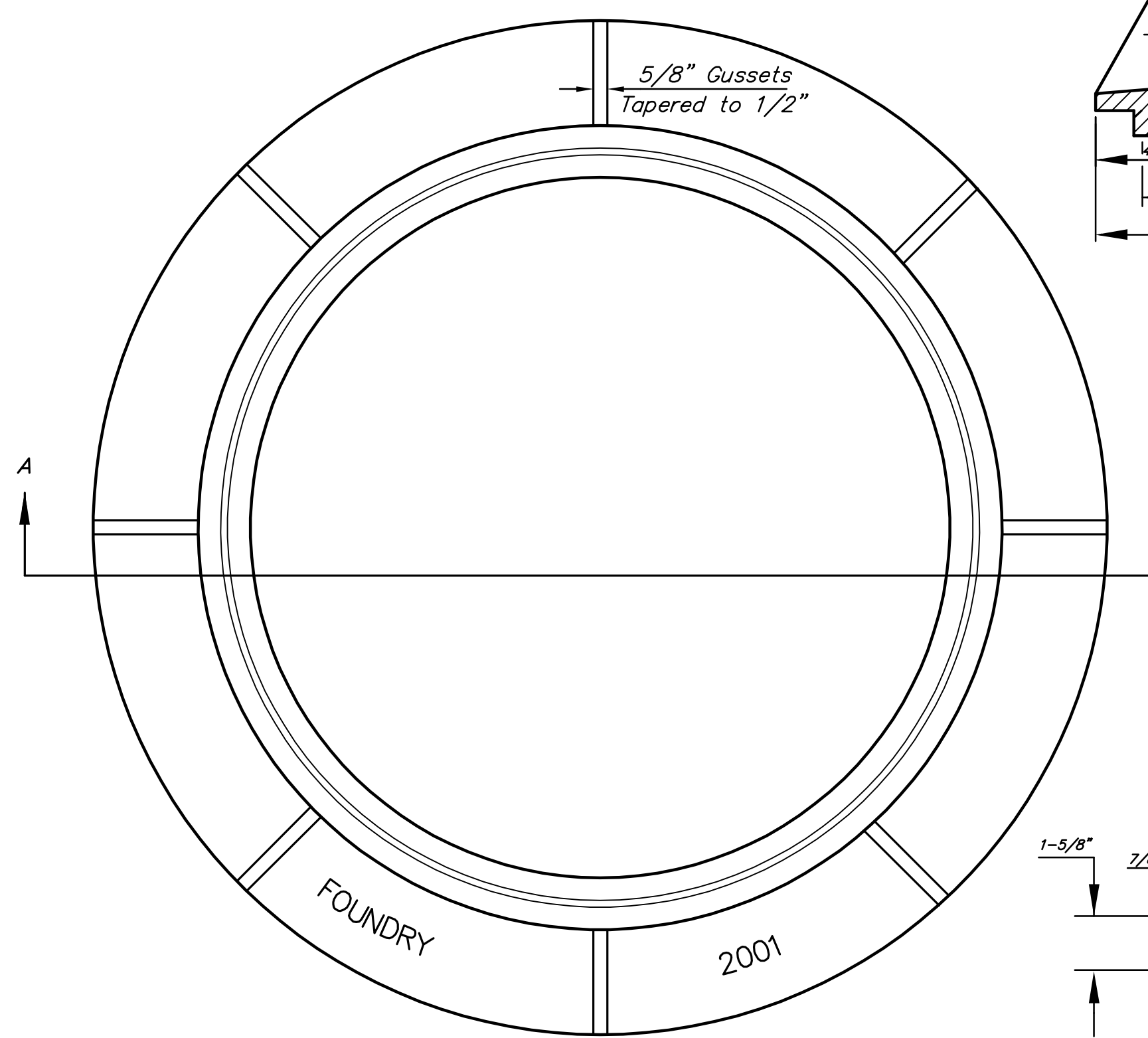
TOP VIEW
