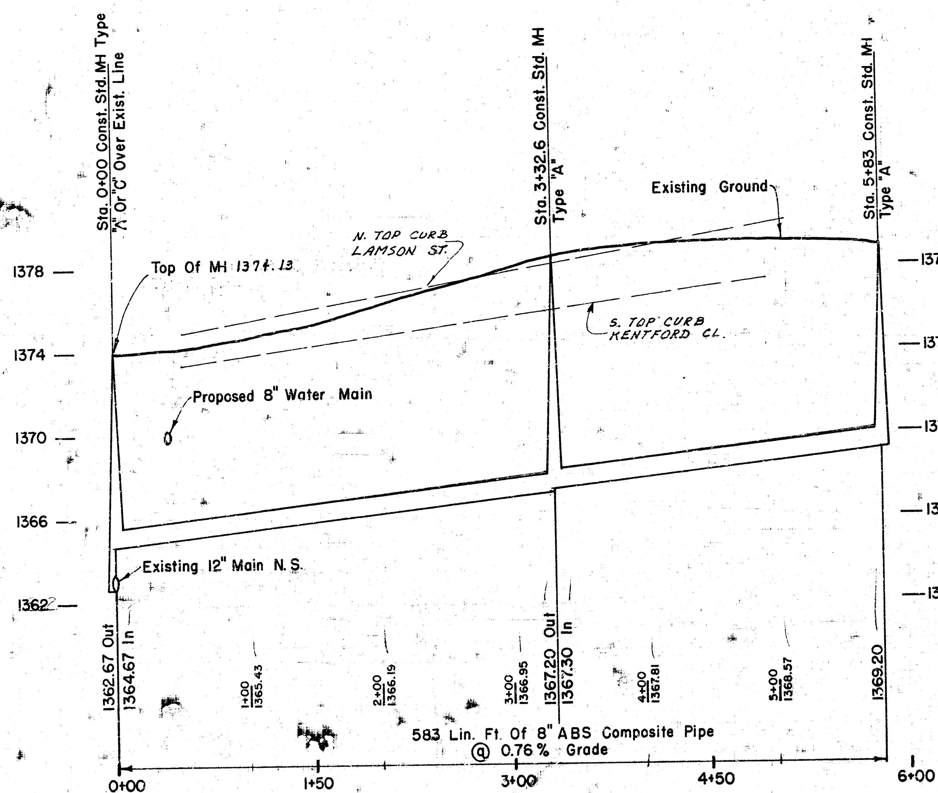
Lateral A Scale 1" = 60' Horiz. 1" = 4' Vert.
