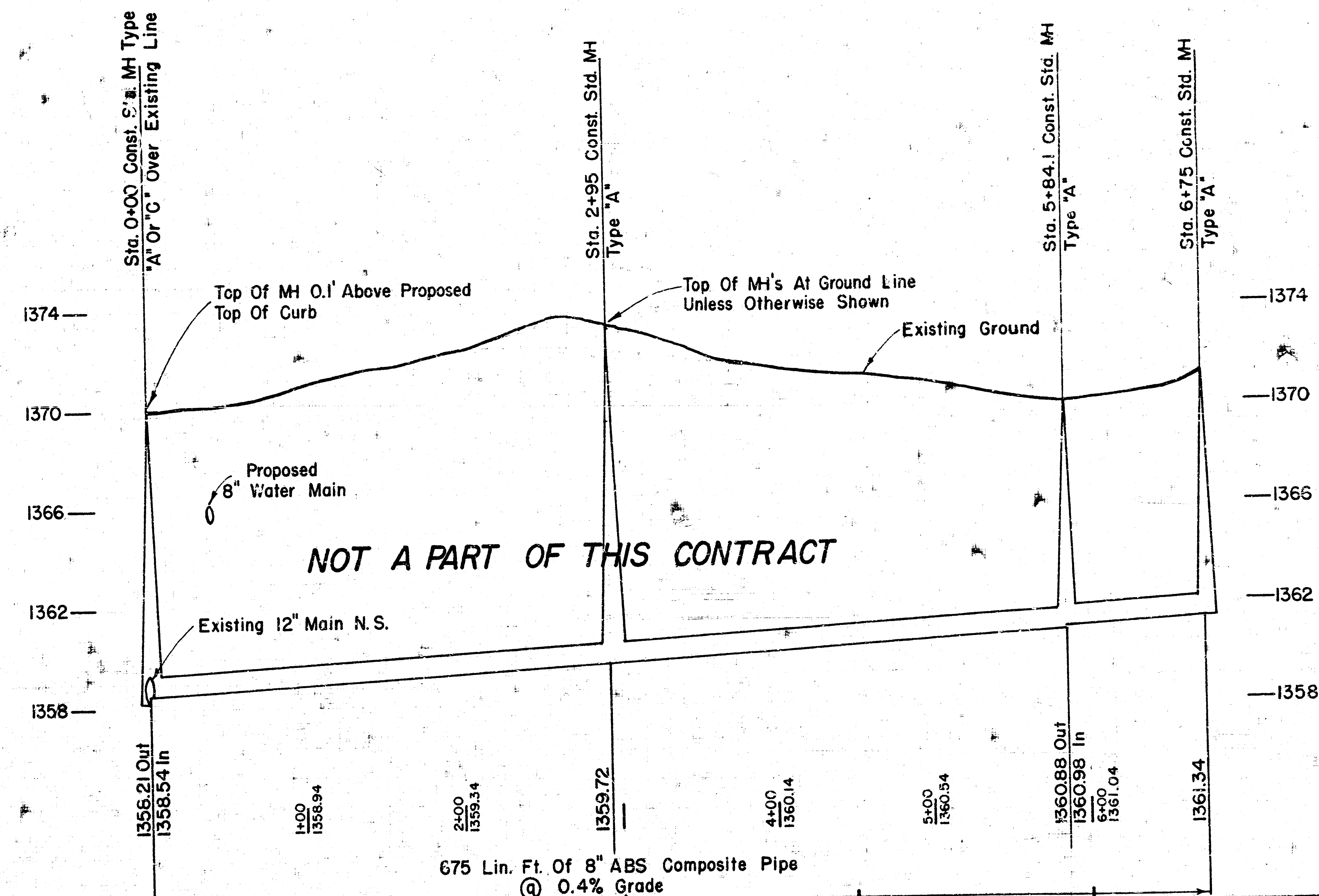
Lateral B Scale 1" = 60' Horiz. 1" = 4' Vert.
