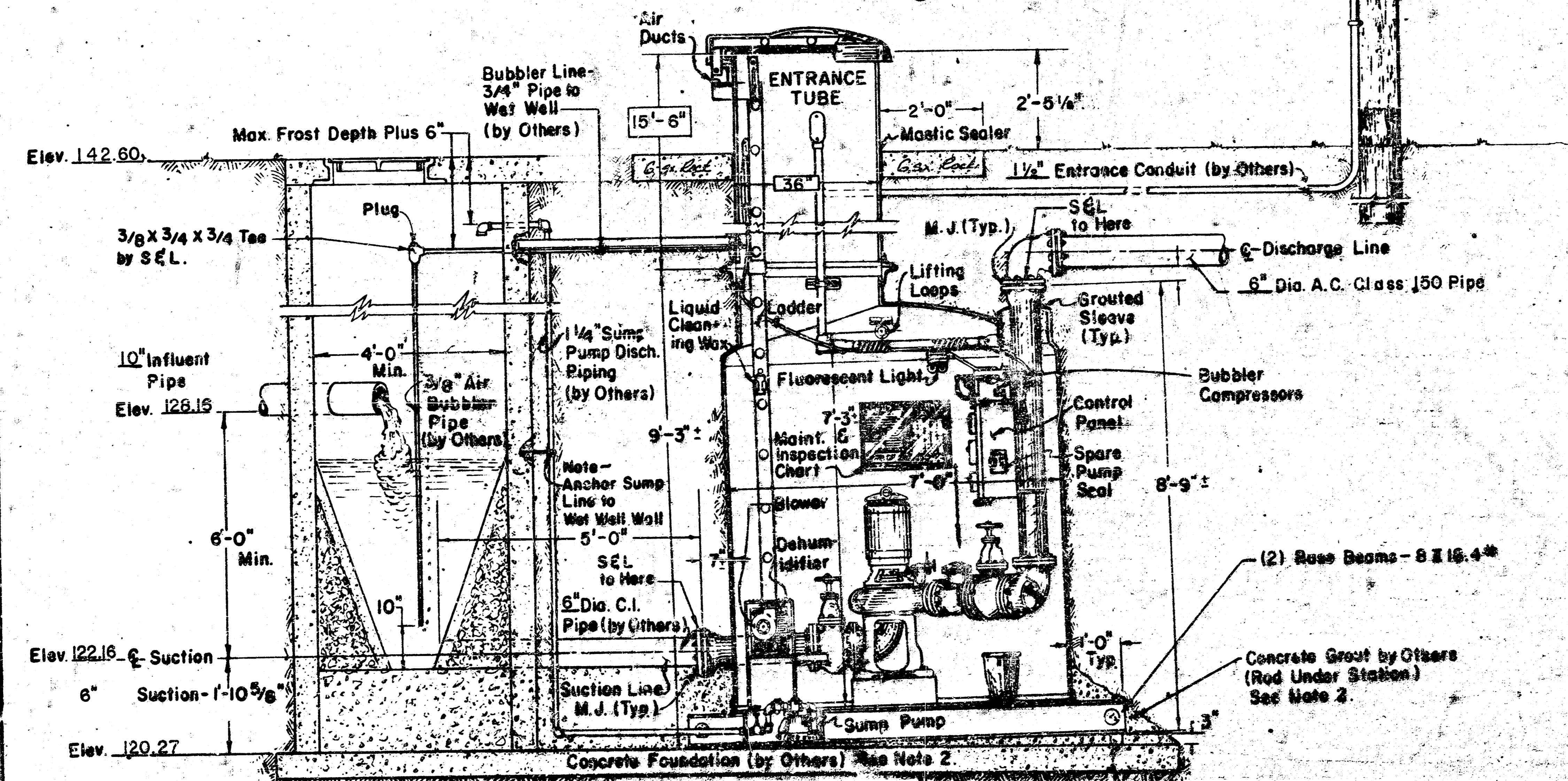
TYPICAL WET WELL (by Others) See Note 2
