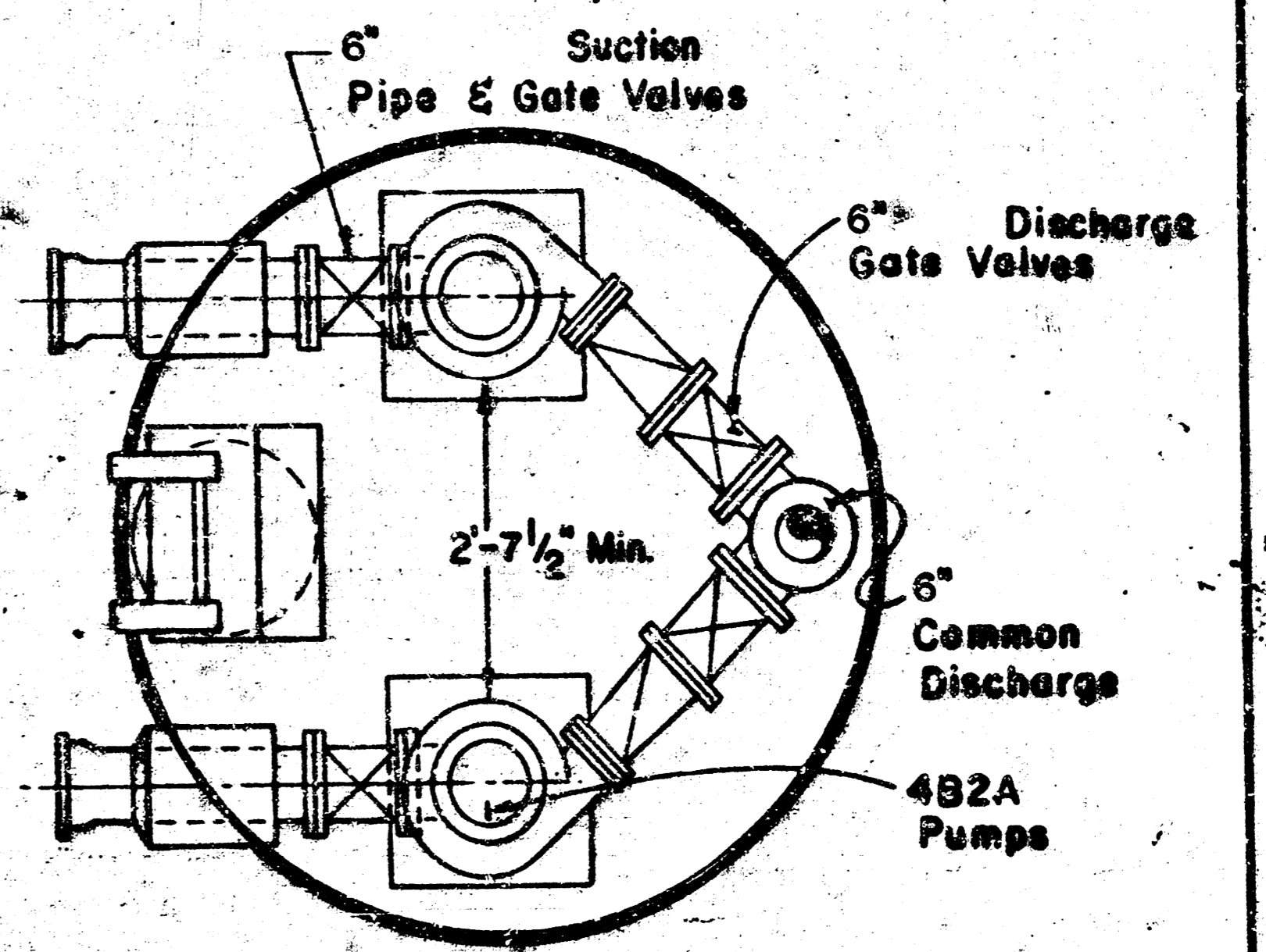
STATION PLAN IN CONNECTION WITH LAT. 7, SOUTHWEST MAIN FLOYD BAILEY ADDITION PRIVATE PROJECT
