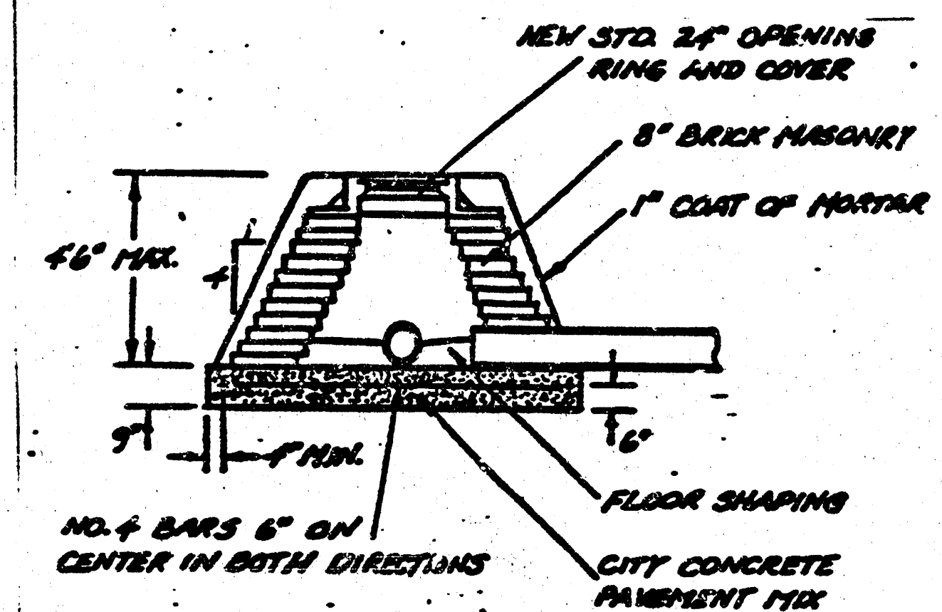
SPECIAL MANHOLE "TYPE A"
