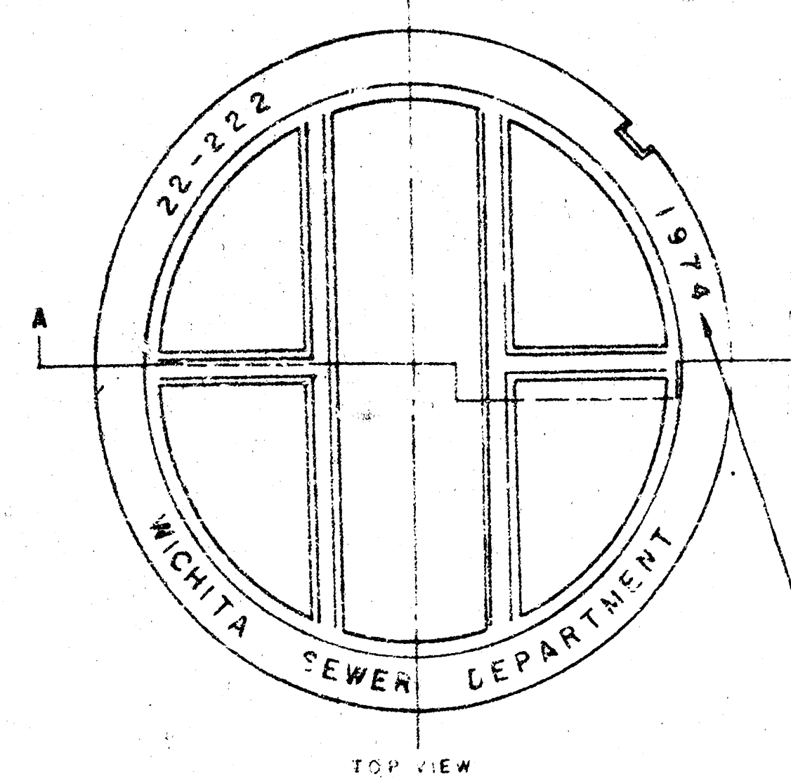
MANHOLE COVER
