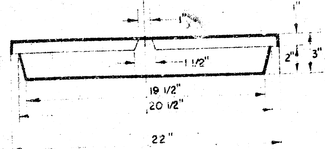
MANHOLE COVER
