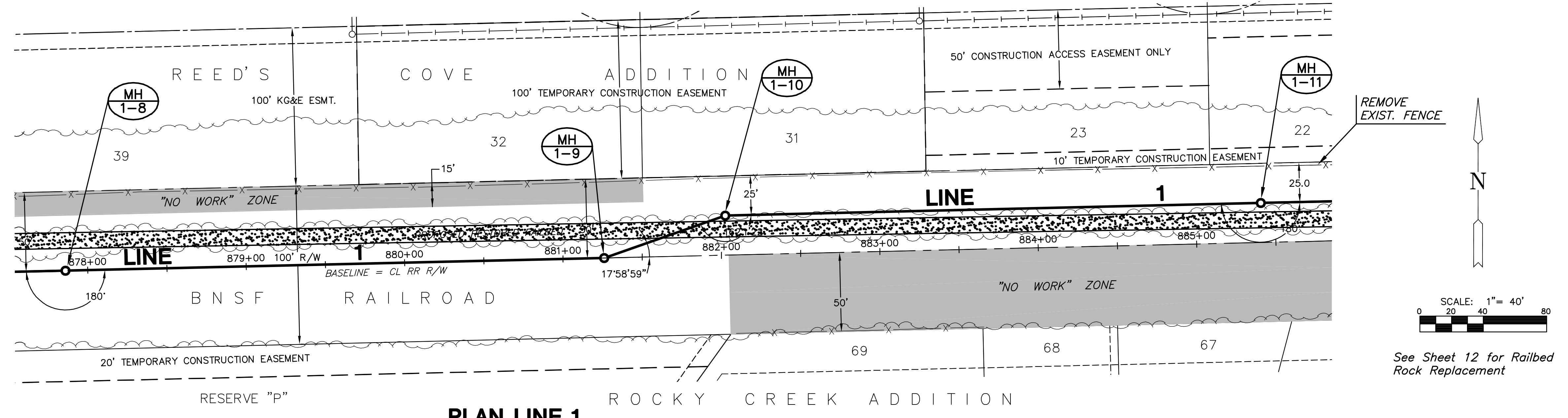
PLAN LINE 1
