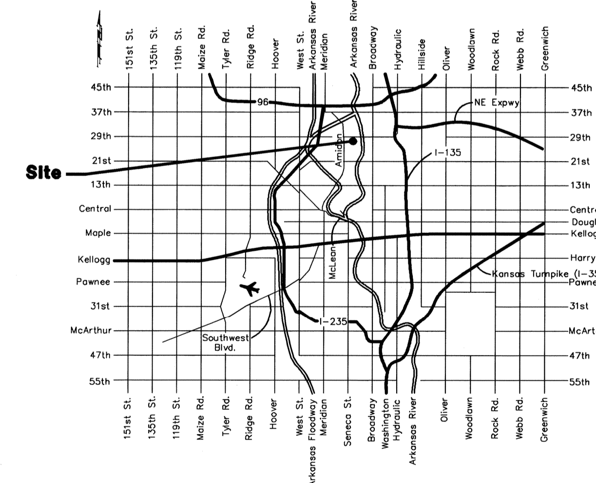
Vicinity Map
